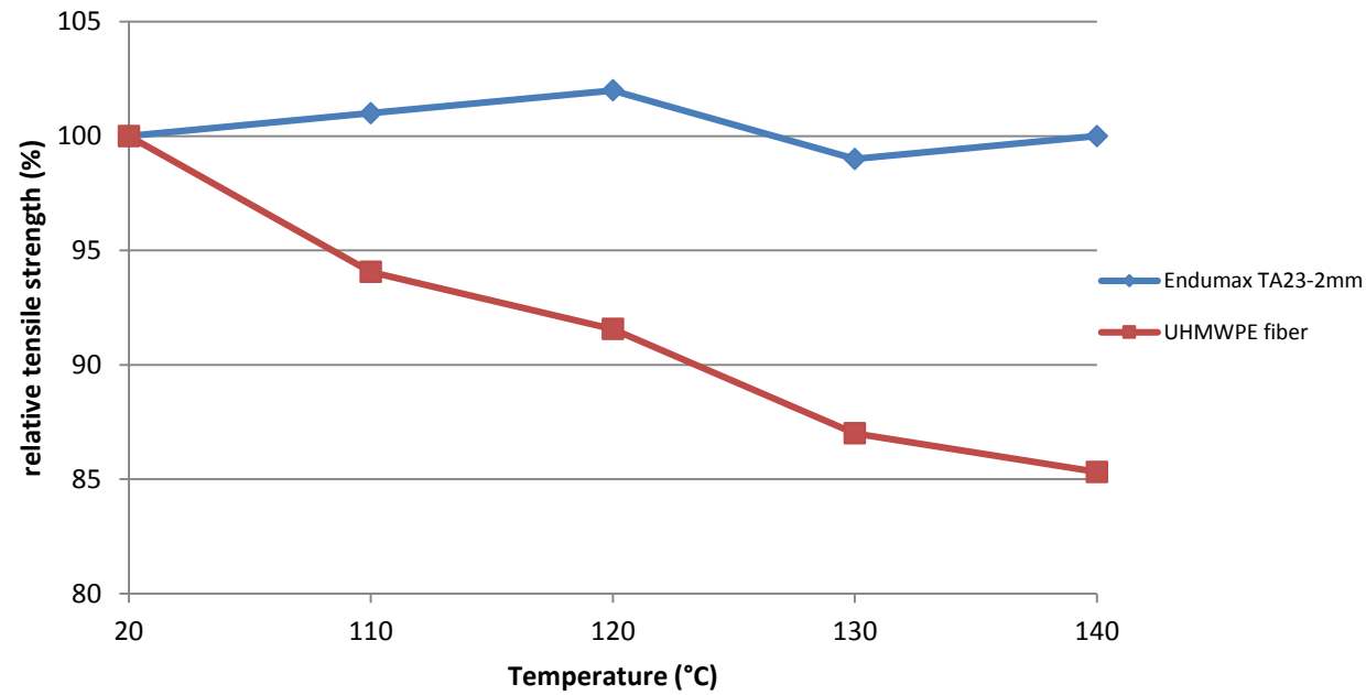
Short time heating: strength retention vs temperature
