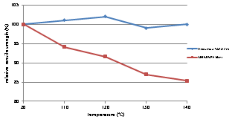
Short time heating: strength retention vs temperature
